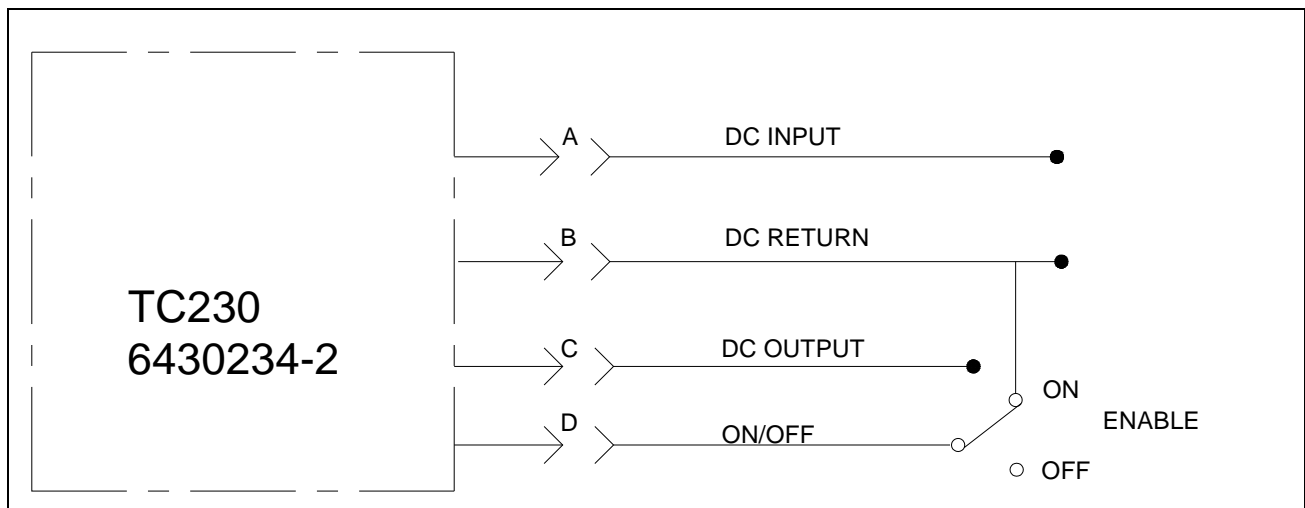
Figure 3.6: Typical 6430234-2 Aircraft Wiring Installation – Remote On/Off
